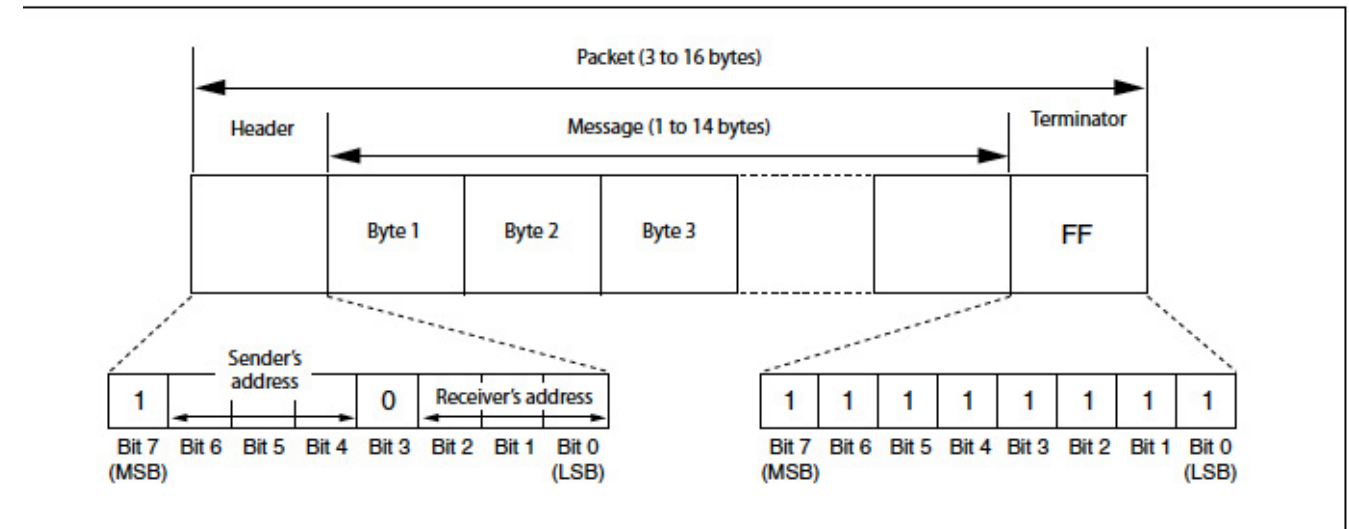
Pic. 1 Packet structure
