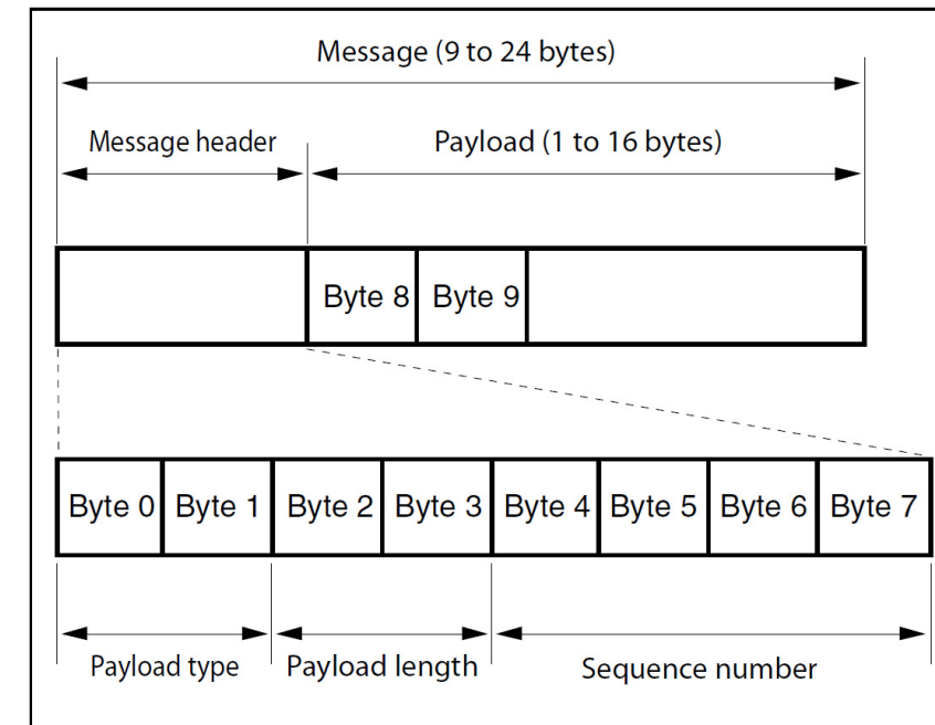
Note: The actual LAN out method is big-endian, LSB first. Pic.3 Message structure of the VISCA over IP
